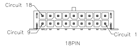
18PIN
