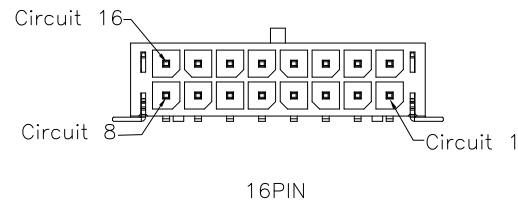
16PIN
