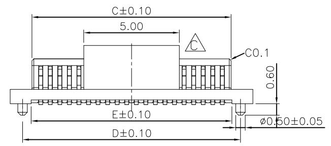
Mating Drawing (Ref)
